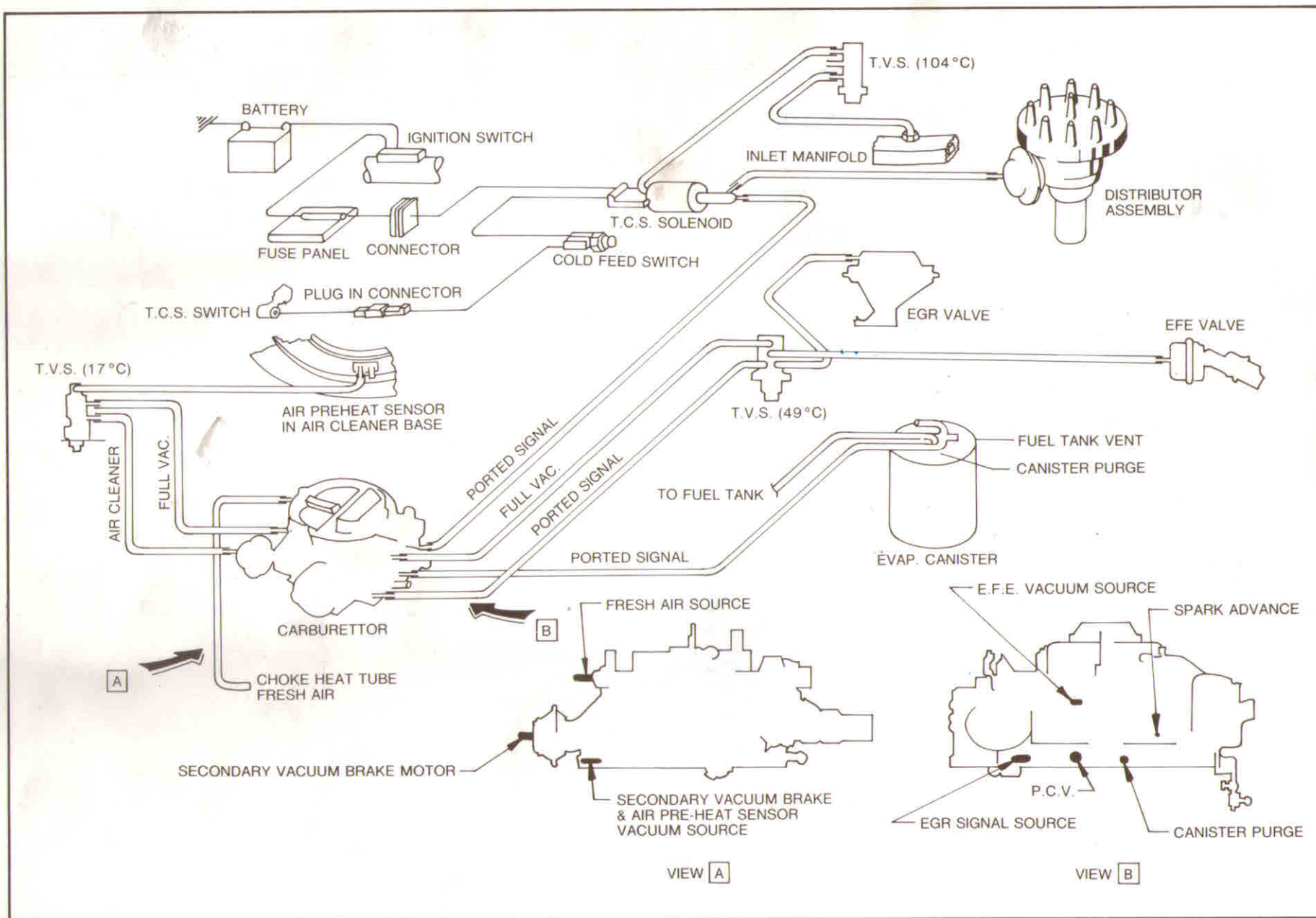
Figure 9-2 8 Cyl. Emission Systems (Schematic)
